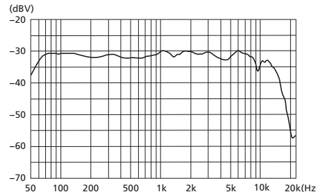
③ Frequenzgang • Frequency response
